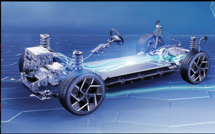
Safety - E-Platform 3.0 With The Cell-to-Body (CTB) Structure
